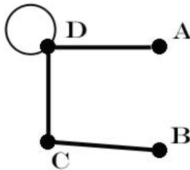
Figure 1. The General Form of \Gamma(Z_{p^2q}) .
