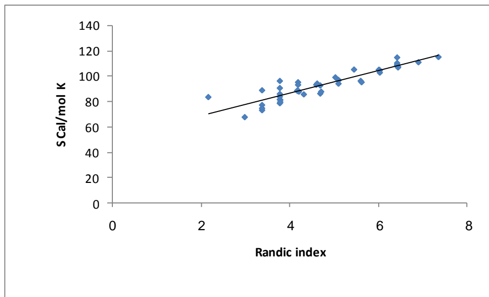
Figure 2. Plots of the Randić index ( {}^1\chi ) versus entropy of 45 benzene derivatives.
