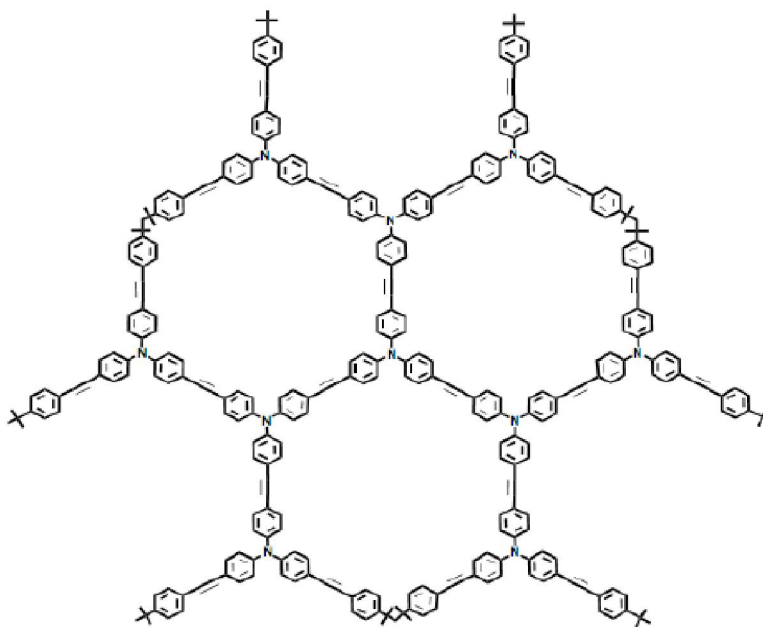
Figure 2. The molecular graph of NSB[2].
