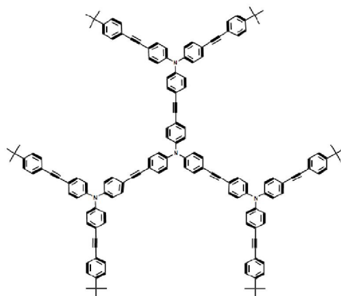
Figure 1. The Molecular Graph of NSB[1].
